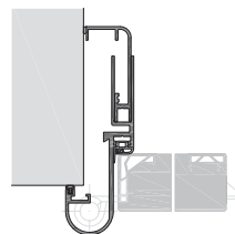
EUROFI-E Eckzarge
